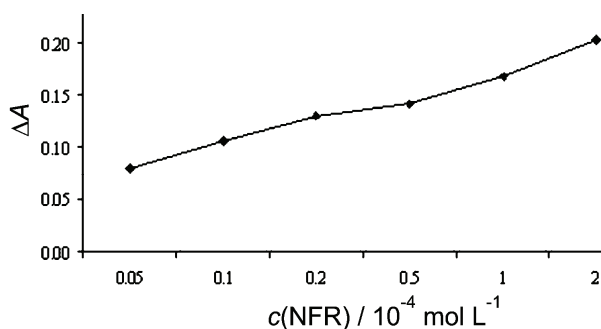
Fig. 2. Effect of the nuclear fast red concentration on \Delta A . Conditions: 10 \mu\text{g mL}^{-1} nitrite; 0.20 \text{ mol L}^{-1} sulfuric acid; 0.020 \text{ mol L}^{-1} potassium bromate; temperature: 25 \text{ }^\circ\text{C} ; reaction time: 5 min.
